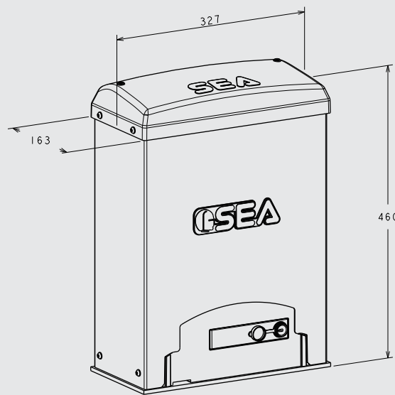
DIMENSIONS (mm)
