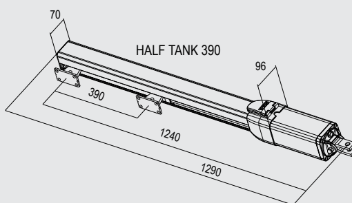
DIMENSIONS (mm)
