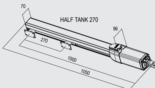
DIMENSIONS (mm)
