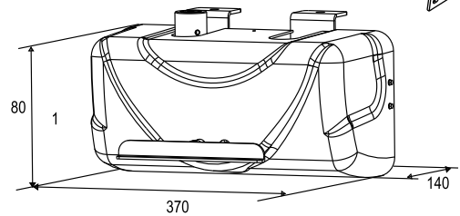
DIMENSIONS (mm)
